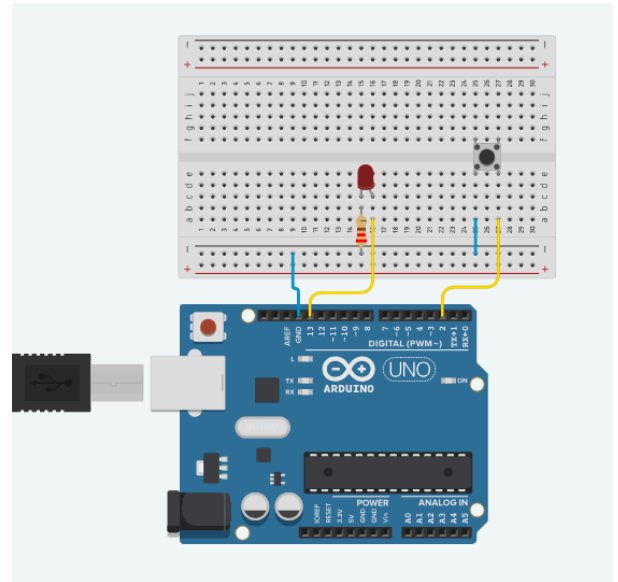
Gambar 3.3 Wiring Percobaan 6A
